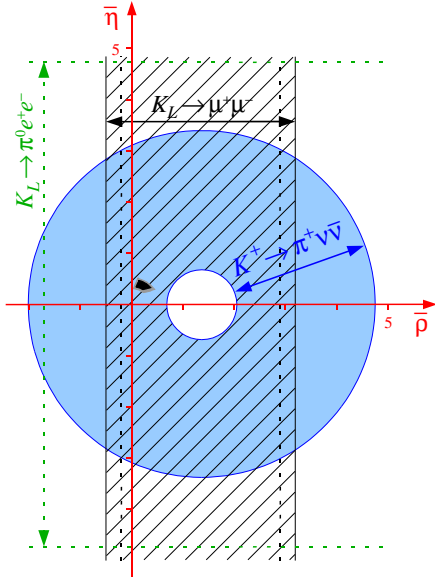
Figure 6. Present constraints in the \bar{p} - \bar{\eta} plane from rare K decays (see text). The small dark region close to the origin denotes the constraints from B -physics and \epsilon_K (see Fig. 1).
