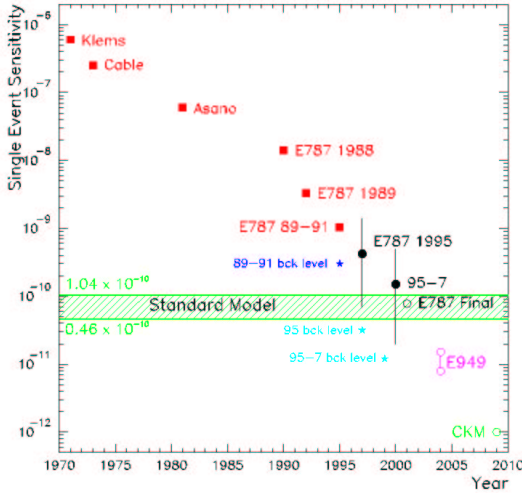
Figure 4. History and future prospects in the experimental search for K^+ \rightarrow \pi^+ \nu \bar{\nu} . 26
