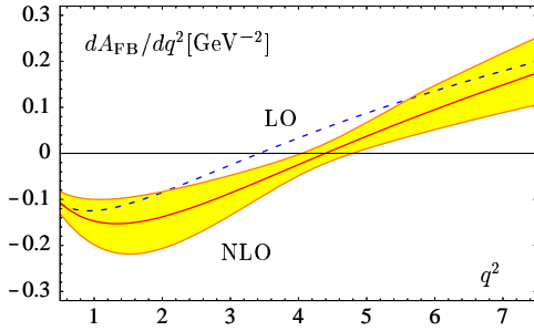
Figure 9. Forward-backward asymmetry of B^- \rightarrow K^{*-} \ell^+ \ell^- at LO and NLO. The band reflects all theoretical uncertainties from parameters and scale dependence combined. 79
